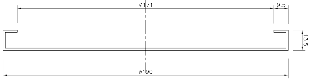
VIEW "A"
